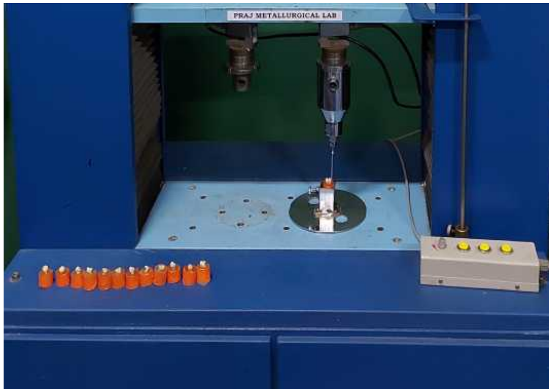
FIGURE 8: SAMPLE SUBJECTED TO LOAD TO MEASURE THE SHEAR BOND STRENGTH
